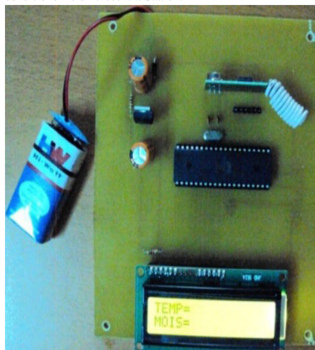
Fig.4:(b) Overview of a Receiver Circuit to connect the LCD display for displaying purpose and Port D is used to connect RF Receiver 433MHz for receiving the data coming from transmitter (field station) to the central station. This data is then sent to microcontroller ATMEGA16. The program is stored in the flash memory of microcontroller. The LCD display is connected to Port C of Controller for displaying the data coming from microcontroller and knows the present condition
